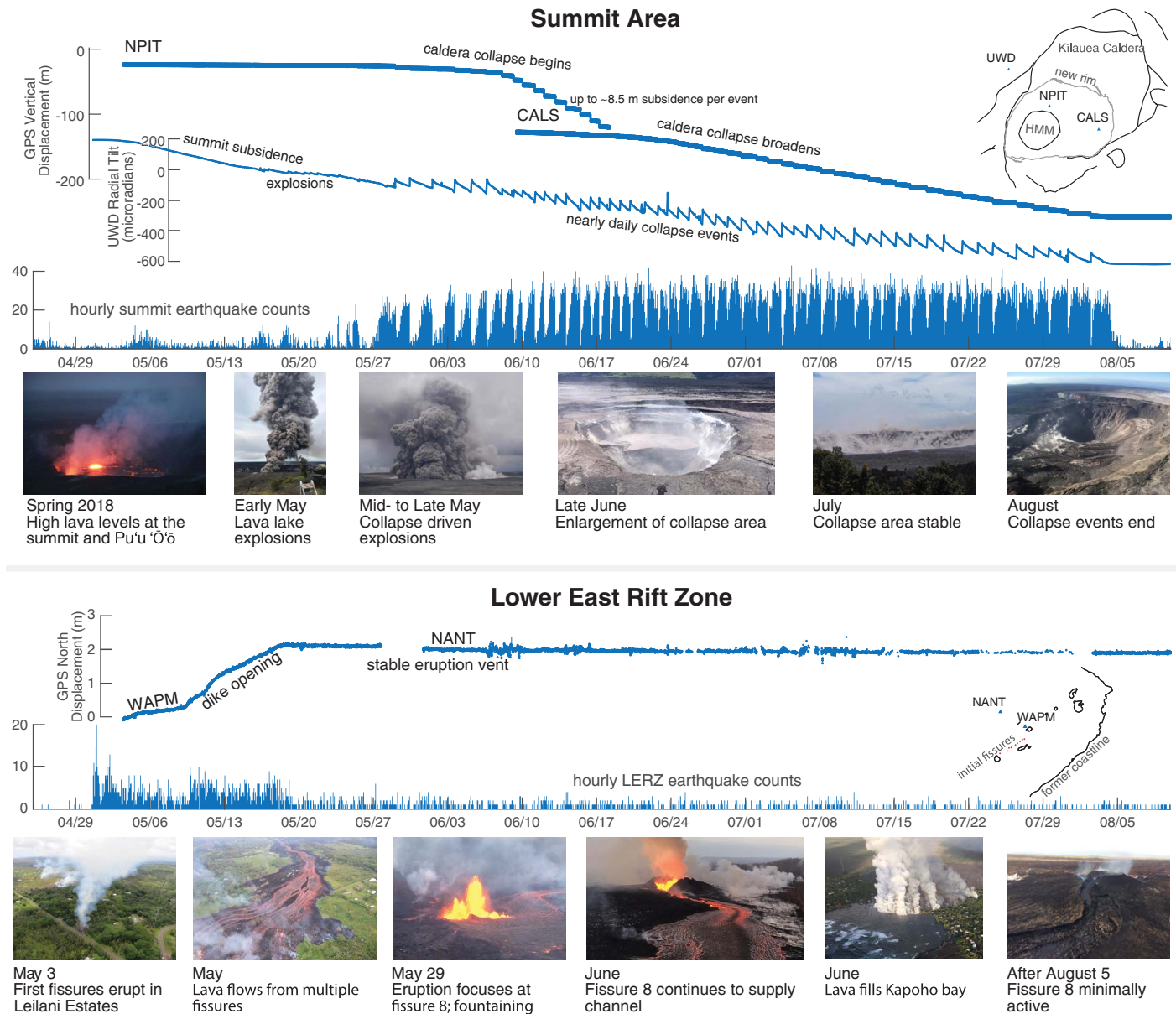
Fig. 2. Timeline of Kilauea's 2018 eruptive activity with representative geodetic and seismic data. On the map, triangles marked with three- and four-letter codes (NPIT, CALS, UWD, WAPM, and NANT) are geodetic station locations. (Top) Activity in the summit area of Kilauea through the time series of GNSS sites located near the initial focus of collapse (NPIT) and farther away (CALS). Near-daily collapse events are manifested as spikes on the UWD tiltmeter and in hourly summit-area earthquake counts.
