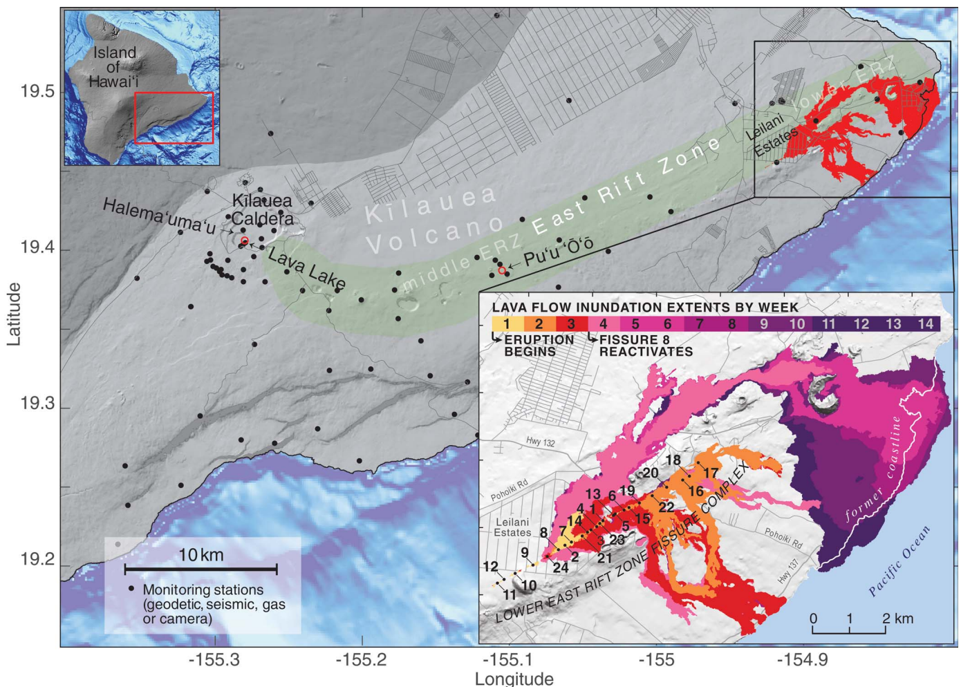
Fig. 1. Map showing the location of Kilauea Volcano on the island of Hawai'i and the general geographic features of the volcano. Kilauea Volcano is indicated in light gray. Gray lines are roads, and dots mark the locations of monitoring stations (geodetic, seismic, gas, or camera). Locations of summit and Pu'u 'Ō'ō eruptive vents are indicated with red
